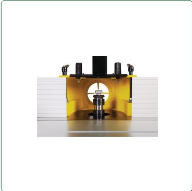
Milling spindle with 80 mm usable length and 30 mm diameter
