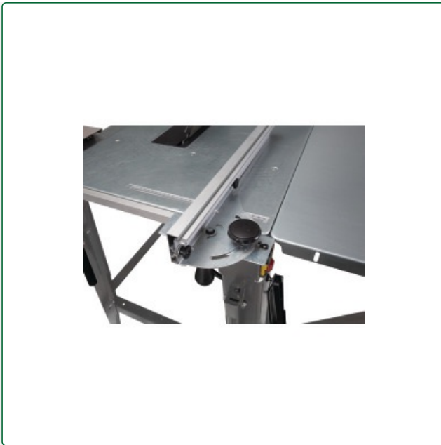
Easy and precise adjustment of the rip fence with eccentric quick tension by scale
